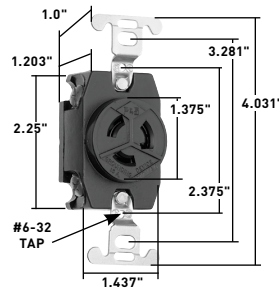
Dimensions for 4760
