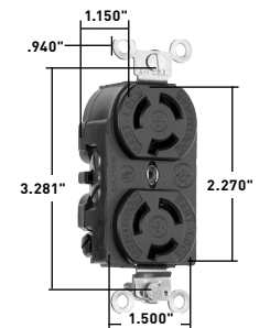
Dimensions for 4550
