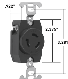
Dimensions for 4560
