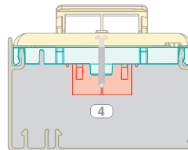
Cable fill #2: Power pole with data terminals using sloped screw-on communication faceplate.
