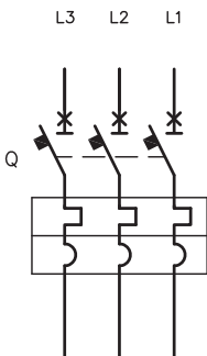
Three-pole circuit-breaker with thermomagnetic trip unit
