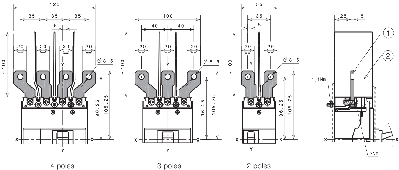
Caption ① Front extended spread terminals ② 100mm insulating barriers between the terminals (compulsory) supplied
