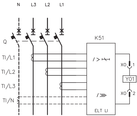
Three-pole/four-pole circuit-breaker with electronic trip unit
