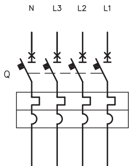
Four-pole circuit-breaker with thermomagnetic trip unit
