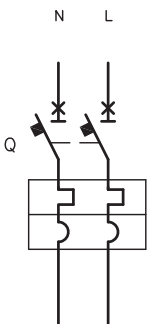
Two-pole circuit-breaker with thermomagnetic trip unit
